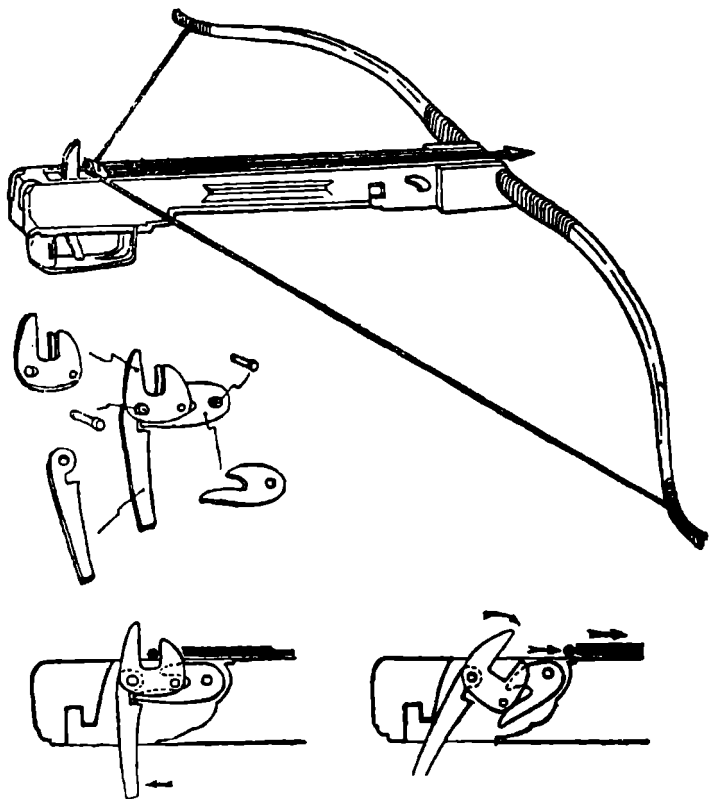
Line drawing of a crossbow and its trigger device dating from the Warring States period (403–221 B.C.) unearthed in a 1952 excavation at Ch'ang-hsia Tomb #138
